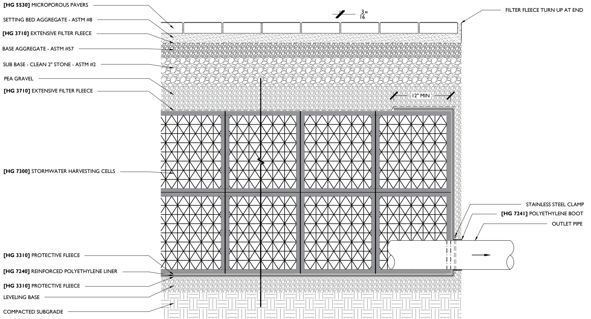
I MICROPOROUS PAVERS OVER STORMWATER CELL RETENTION W/ OUTLET PIPE - DOUBLE LAYER SCALE: 1" = 1'-0"
