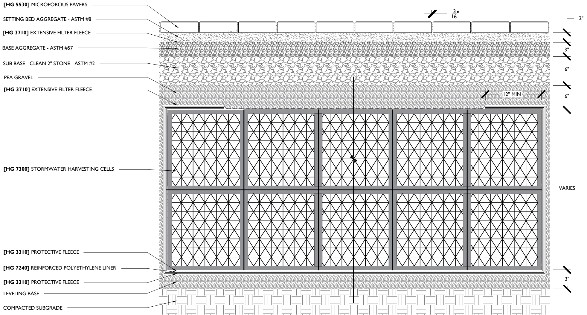
I MICROPOROUS PAVERS OVER STORMWATER CELL RETENTION - DOUBLE LAYER SCALE: 1" = 1'-0"
