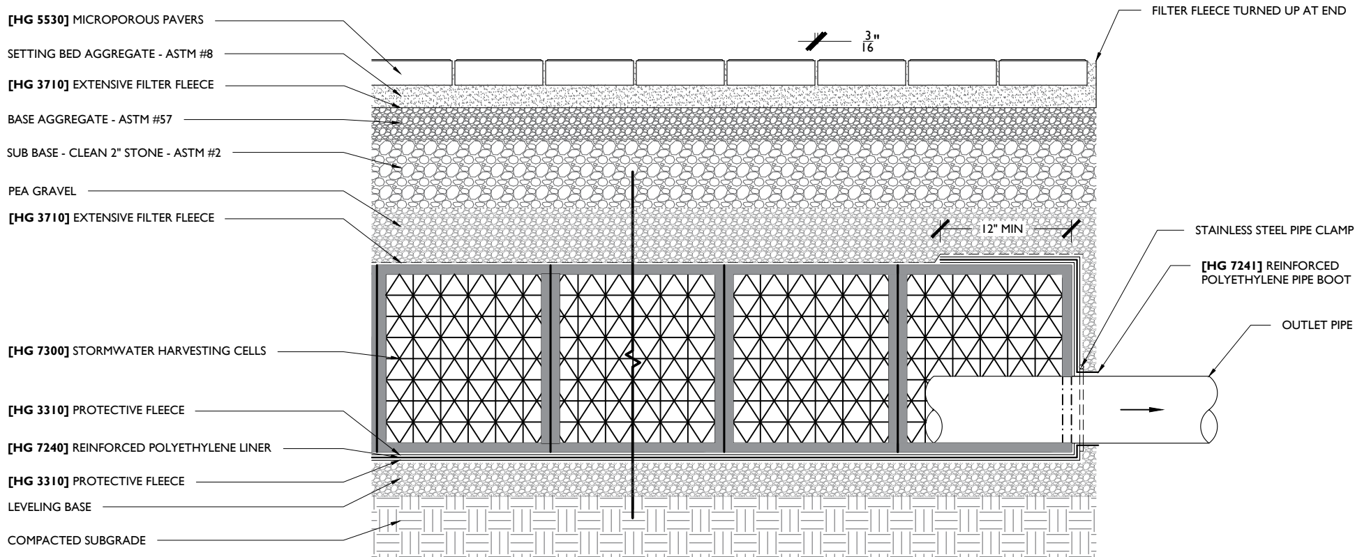
I MICROPOROUS PAVERS OVER STORMWATER CELL RETENTION W/ OUTLET PIPE - SINGLE LAYER SCALE: 1" = 1'-0"
