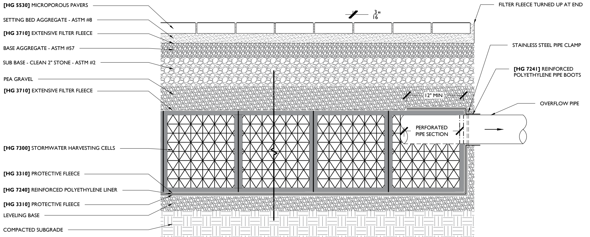
I MICROPOROUS PAVERS OVER STORMWATER CELL RETENTION W/ OVERFLOW PIPE - SINGLE LAYER SCALE: 1" = 1'-0"
