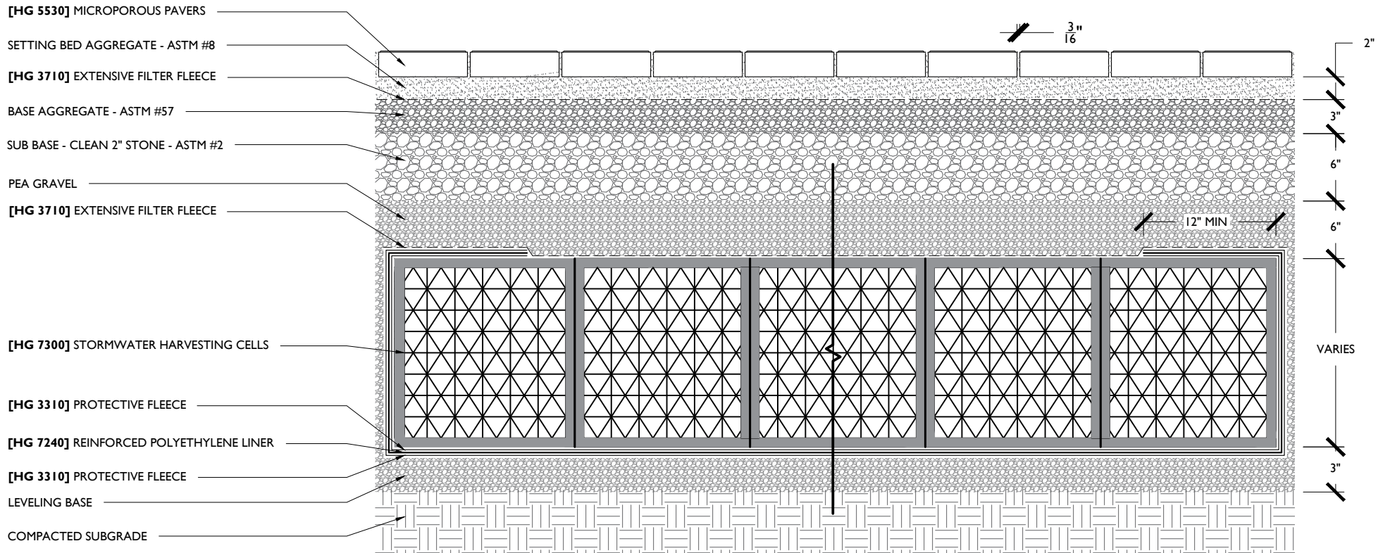
I MICROPOROUS PAVERS OVER STORMWATER CELL RETENTION - SINGLE LAYER SCALE: 1" = 1'-0"
